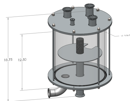
High Performance Bubble Trap
